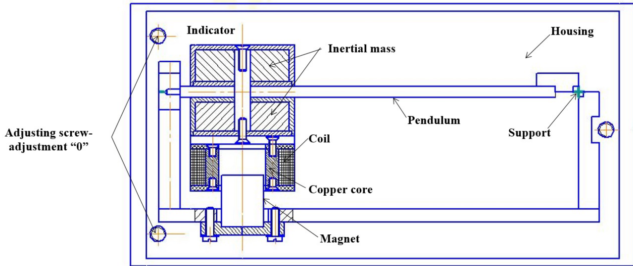
Figure 2. Structural diagram of the seismic sensor IGES-006.
