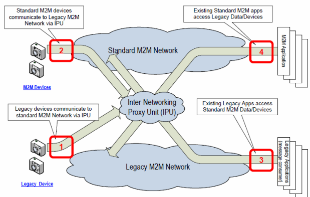
Figure 5. M2M internetworking
