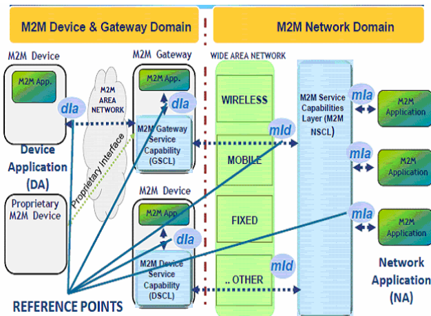
Figure 1. M2M ETSI [7]
